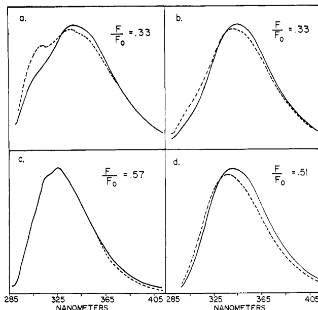
FIGURE 2: Technical fluorescence emission spectra of proteins equilibrated with air and increased oxygen pressure. The fraction of the original fluorescence remaining is listed as F/F_0 . Experimental conditions are listed in the footnotes to Table II: (a) human serum albumin; (b) bovine serum albumin; (c) aldolase; (d) carbonic anhydrase.
