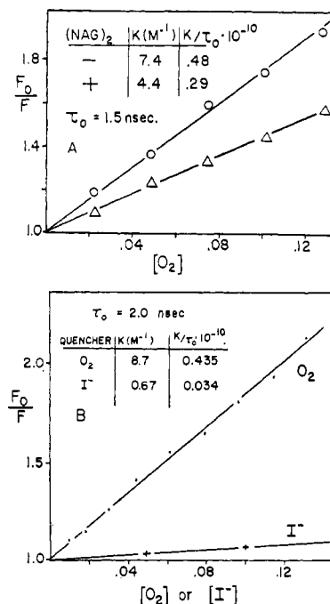
FIGURE 4: (a) Oxygen quenching of lysozyme in the presence (Δ) and absence (O) of (N-Ac-GlcN) 2 ; 0.1 M sodium phosphate, pH 7; 280-nm excitation, 340- (no (N-Ac-GlcN) 2 ) or 330-nm (with (N-Ac-GlcN) 2 ) emission; [lysozyme] = 7.6 \times 10^{-5} M, [(N-Ac-GlcN) 2 ] = 3.2 \times 10^{-3} M. (b) Comparison of oxygen and iodide quenching of trypsinogen; O 2 quench: 0.001 M HCl, 280-nm excitation; I - quench: 0.001 M HCl, 290-nm excitation, [KCl] + [KI] = 0.50 M, ca. 10^{-4} M Na 2 S 2 O 3 ; 334-nm emission was used for both samples.
